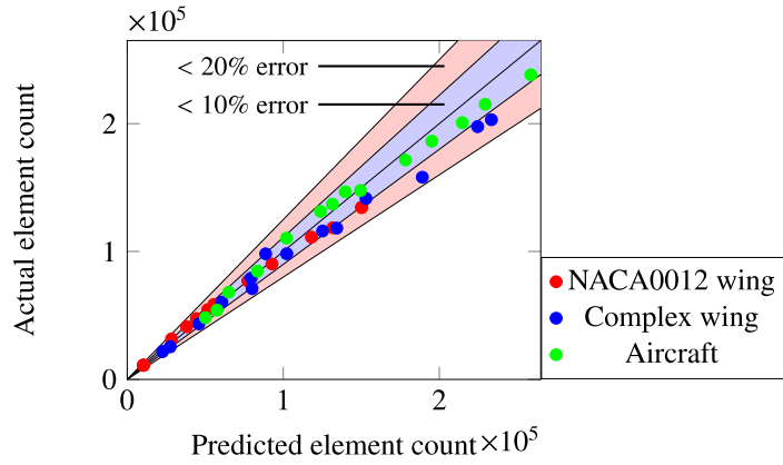
Figure 2: Predicted vs actual element count for various meshes using the automatic octree system
