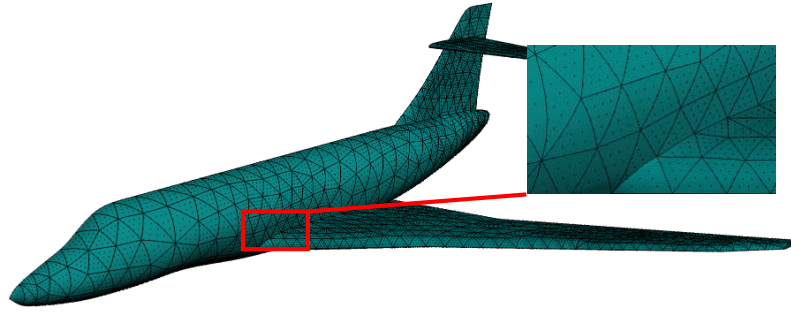
Figure 3: High-order surface mesh of the aircraft geometry.
